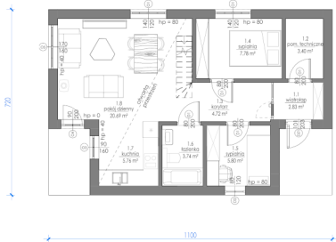
PARTER
